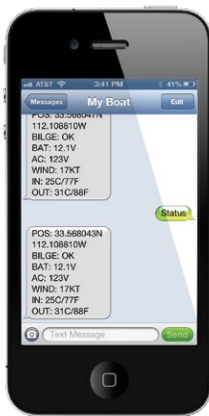
Status Text
