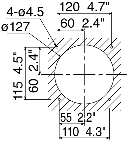
Cutout for flush mount
