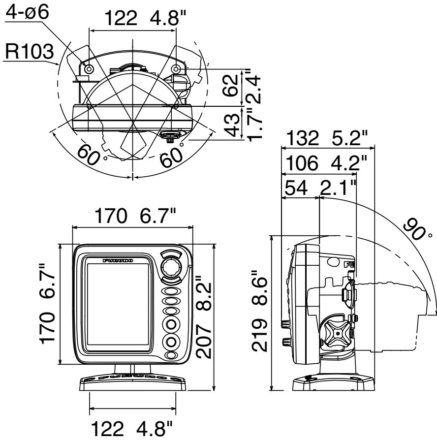
FCV620 Display Unit
