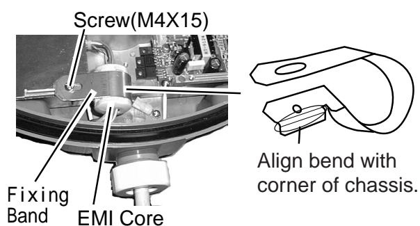
Figure 10 How to fix the EMI Core
