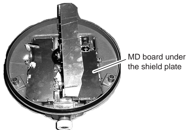
Figure 26 MD board
