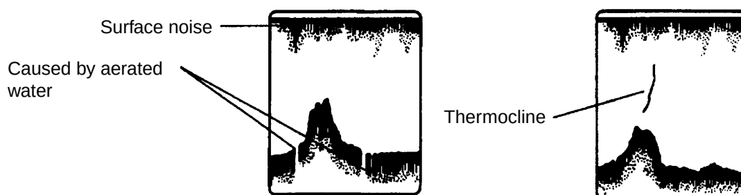
Surface noise/aeration
