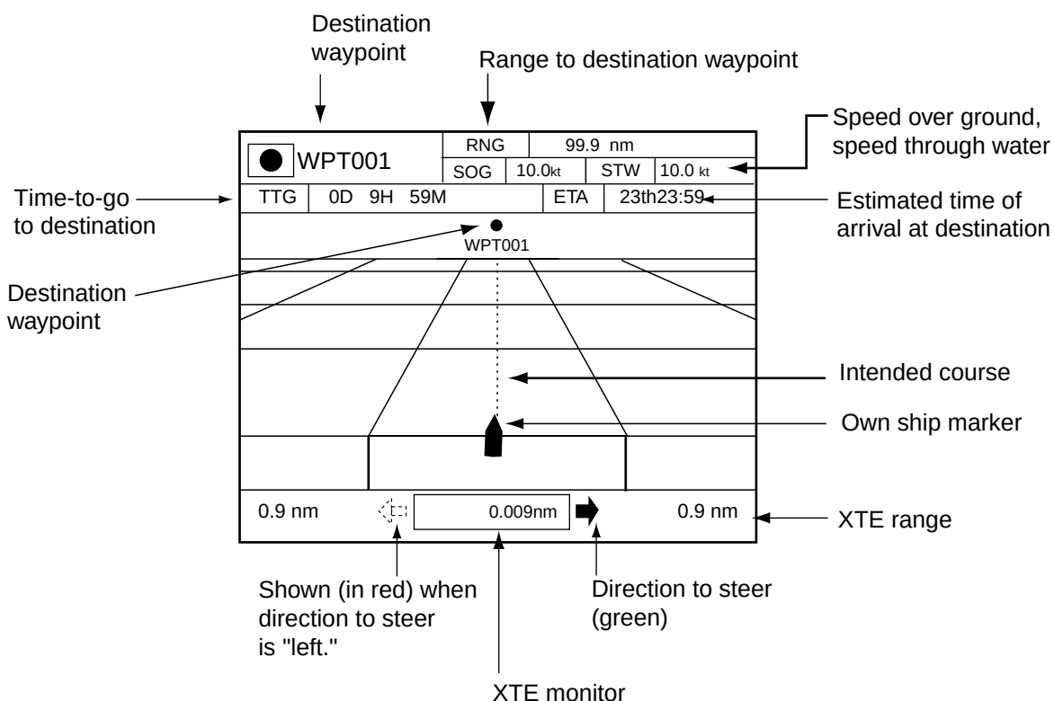
Highway display
