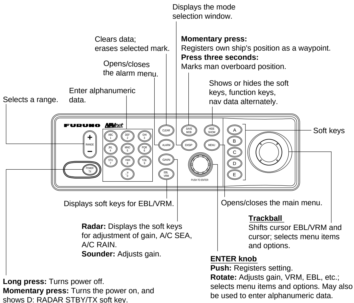
Control unit
