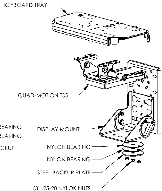
Display Mount, Quad-Motion TS5 & Keyboard Tray
