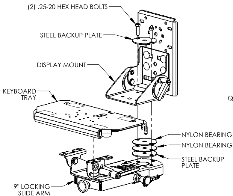
Display Mount, 9" Locking Slide Arm & Keyboard Tray
