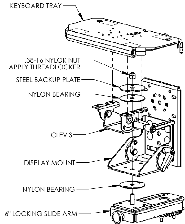
Display Mount, Clevis, 6" Locking Slide Arm & Keyboard Tray
