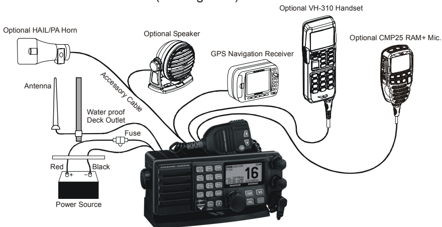
Figure 1. General Installation
